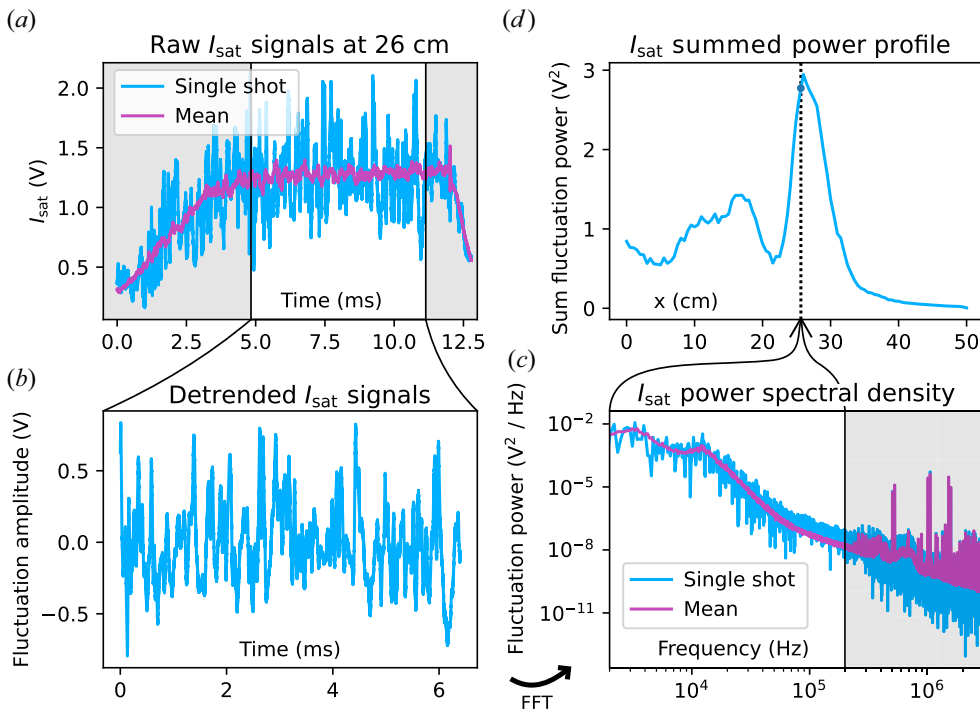
FIGURE 2. Raw data and basic processing steps for LAPD probe diagnostics as demonstrated by an I_{\text{sat}} trace from a DR1, M = 1 mirror at 26 cm. Data are truncated from 4.8 to 11.2 ms (a) and detrended (b). Power spectral density is calculated (c), and a power profiles can be constructed (d). The shaded regions are excluded from this analysis.
