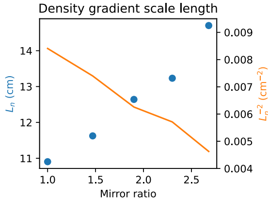
FIGURE 19. Gradient scale length L_n and the associated term in the drift-wave growth rate L_n^{-2} . This scale length was calculated over a 3 cm region around x_{PF} (peak-fluctuation region) at the midplane. Increasing the mirror ratio increases the gradient scale length, which suggests weakening of the underlying instability driver.
